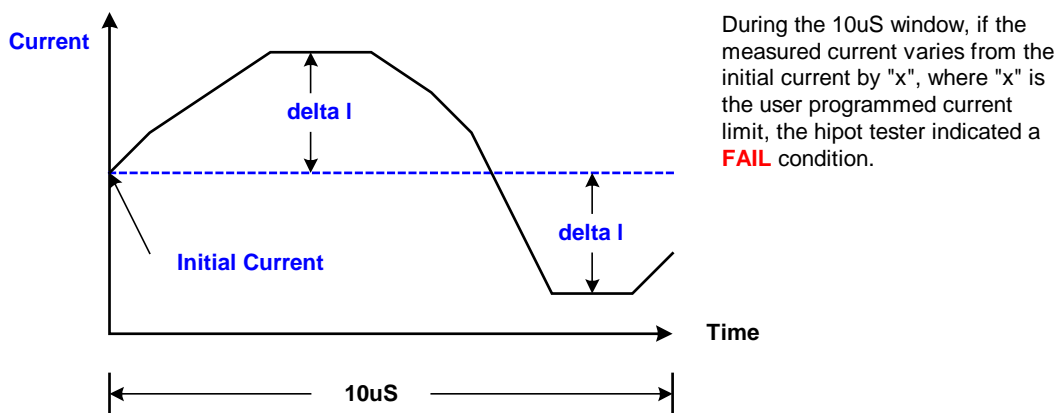
Figure 5: Arc Detection
