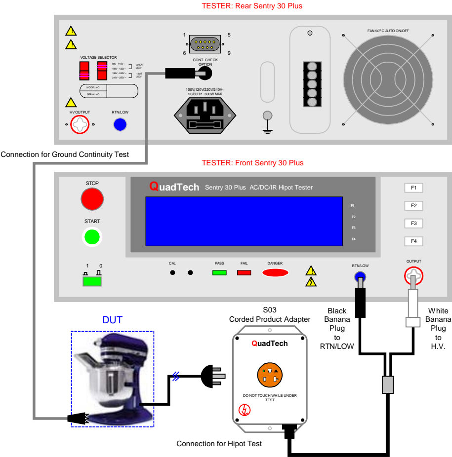
Fig. 7 Connection to DUT for Ground Continuity & Hipot Tests *
