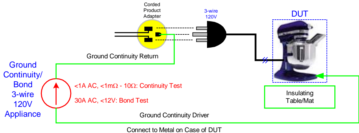
Figure 6. Ground Continuity Test
